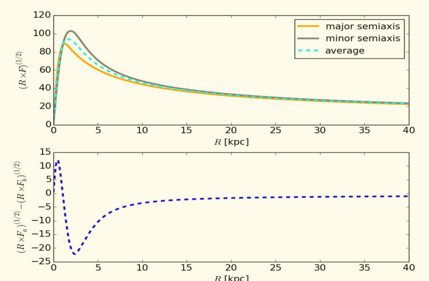
Figure 6: Top: Rotation curve along the major and minor axes for triaxial bar. Bottom: Difference between the two rotation curve major - minor / semiaxis.
